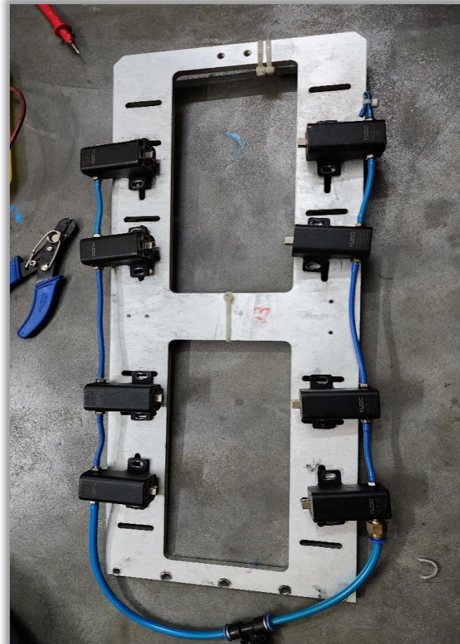
ROBOTIC JIGS
